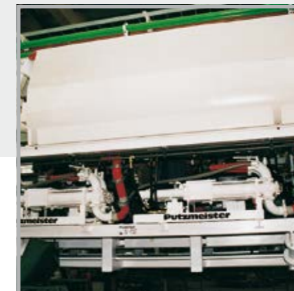
Left: A KOV 1050 pumps the injection mortar behind the ring segment Right: Space-saving installation with two KOV 550 Duo underneath a 6 m 3 agitating trough
