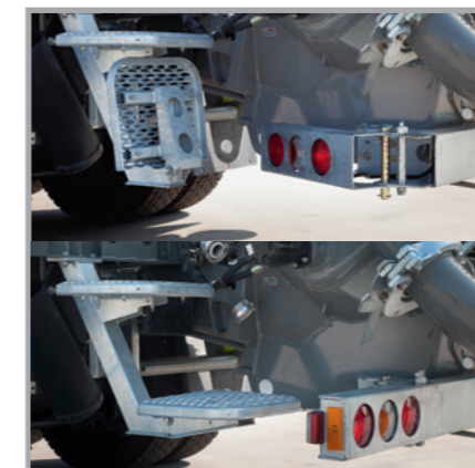
Folding steps in order to prevent damage when filling with two truck mixers.
